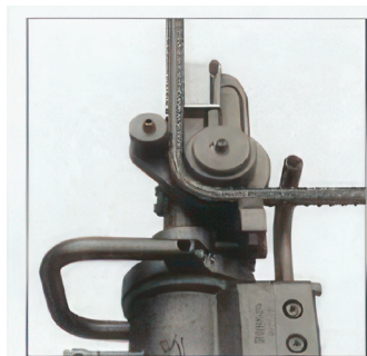
Bending 90°
