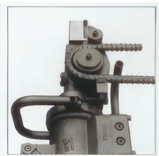
Bending 180°
