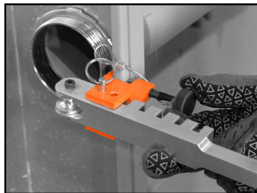
SLOTTED EXTENDER ARM ROLLER TIP with removable & adjustable conduit clamp
