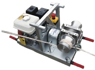
Petrol Twin Capstan (1000kg) - 25m/min
